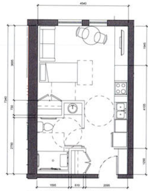
STUDIO - ACCESSIBLE 37 m 2 (398 sf)
