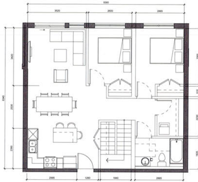
4 BEDROOM - TYPE A @ L1 138 m 2 (1485 sf)
