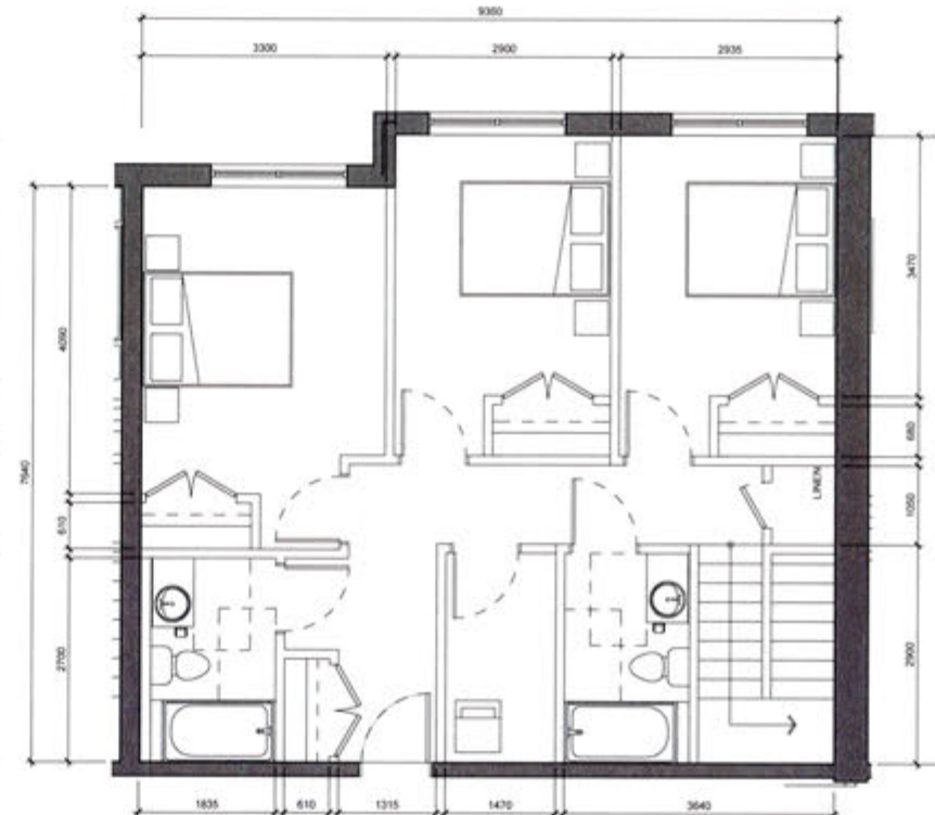
4 BEDROOM - TYPE B @ L2
