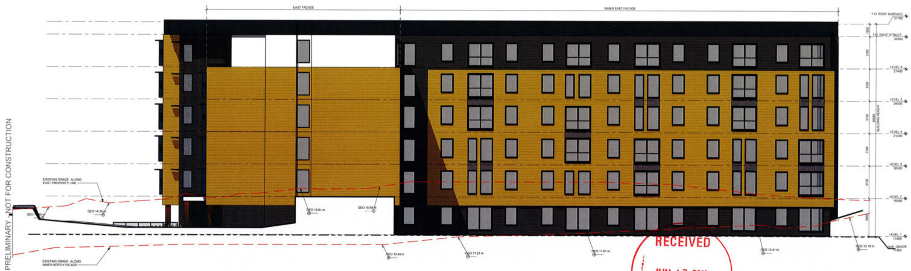
EAST ELEVATION.
