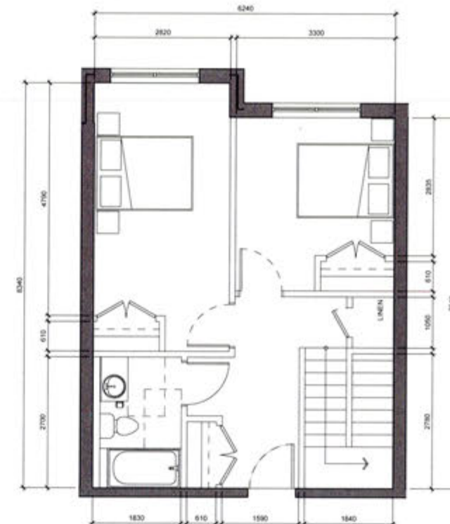
4 BEDROOM - TYPE A @ L2
