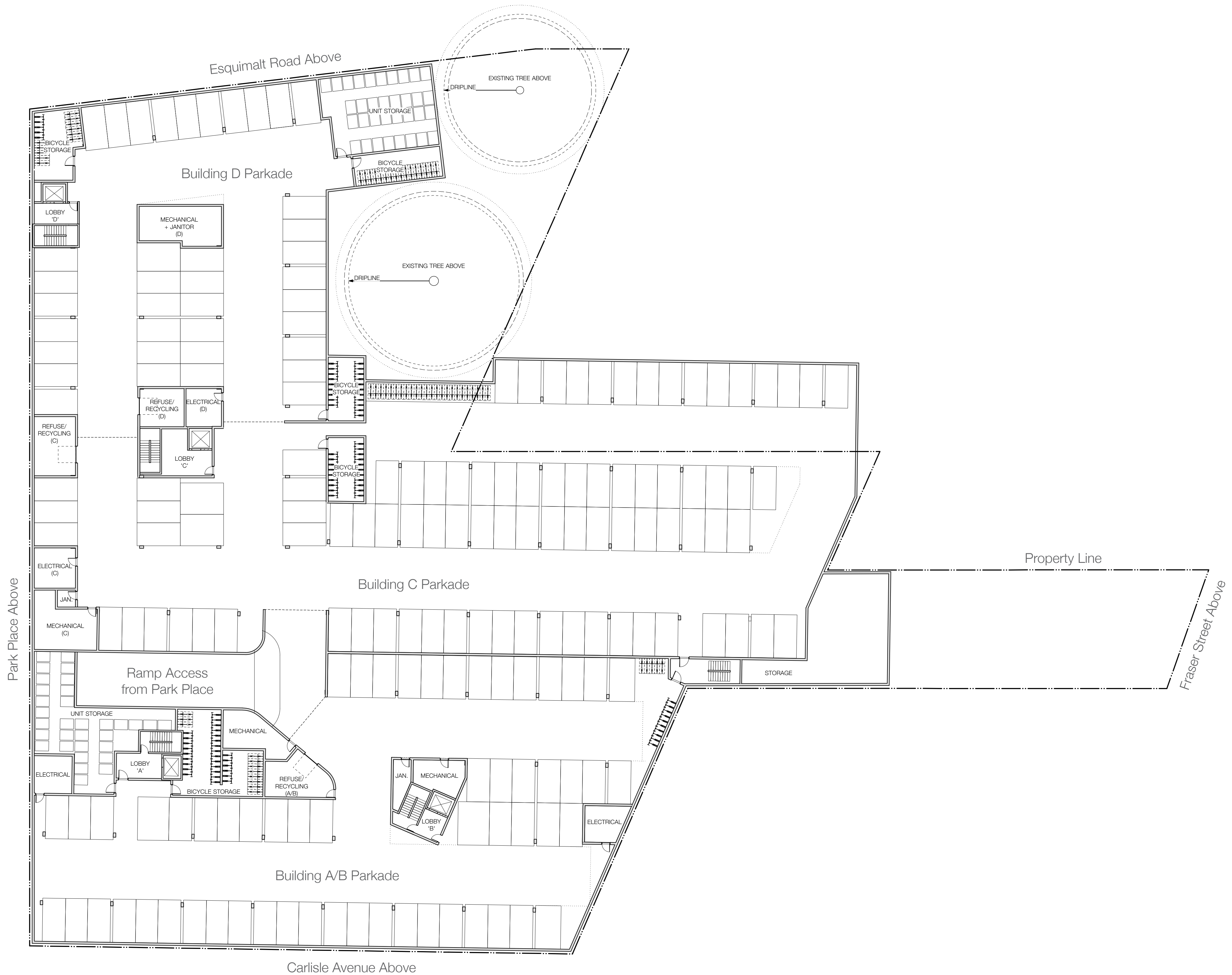
Parking Plan 1:250
