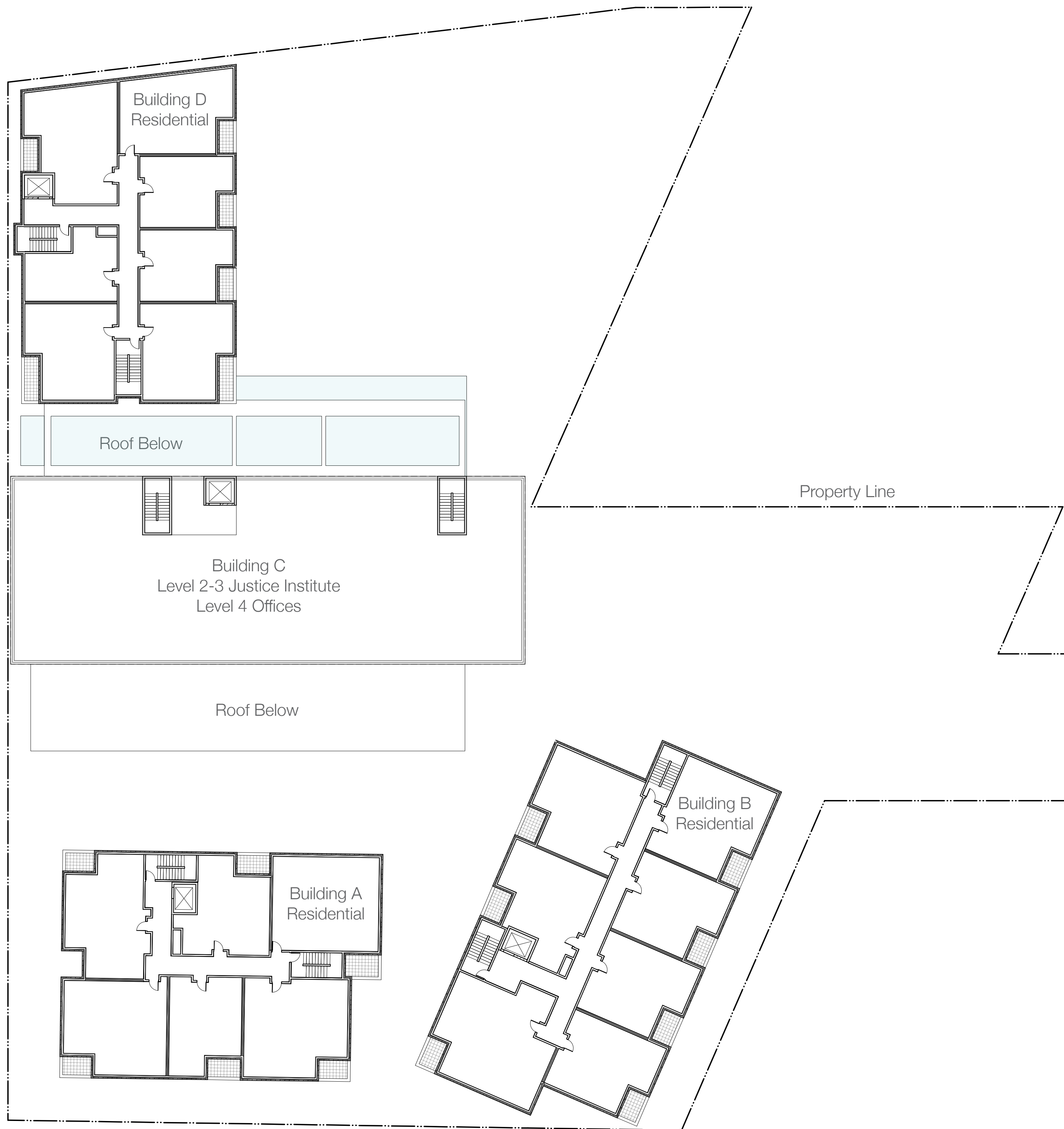
Upper Floor Plan 1:250 Levels 2-4
