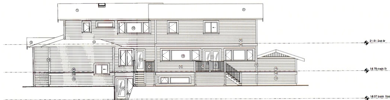
4 South Elevation 1/8" = 1'-0"
