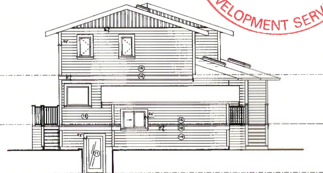
3 East Elevation 1/8" = 1'-0"
