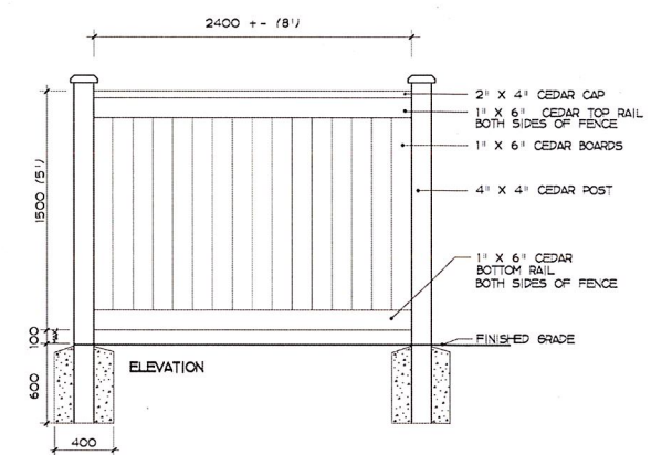
WOOD PERIMETER FENCE
