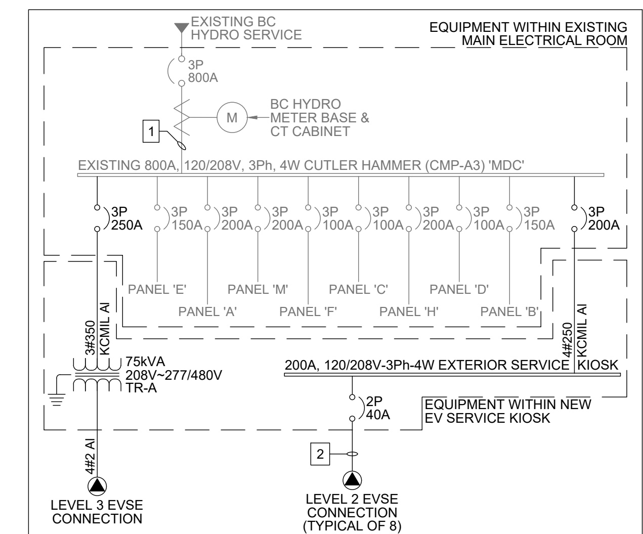
2 SINGLE LINE DIAGRAM E1 SCALE: NTS
